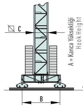
TRAVELLING BASE
