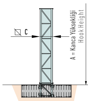
FOUNDATION ELEMENT
