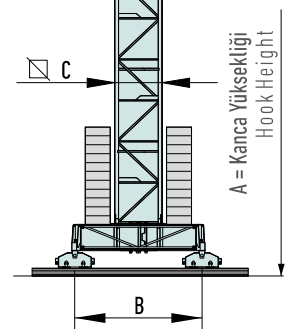
TRAVELLING BASE
